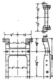
Figs. 3388-3390. Transom.
